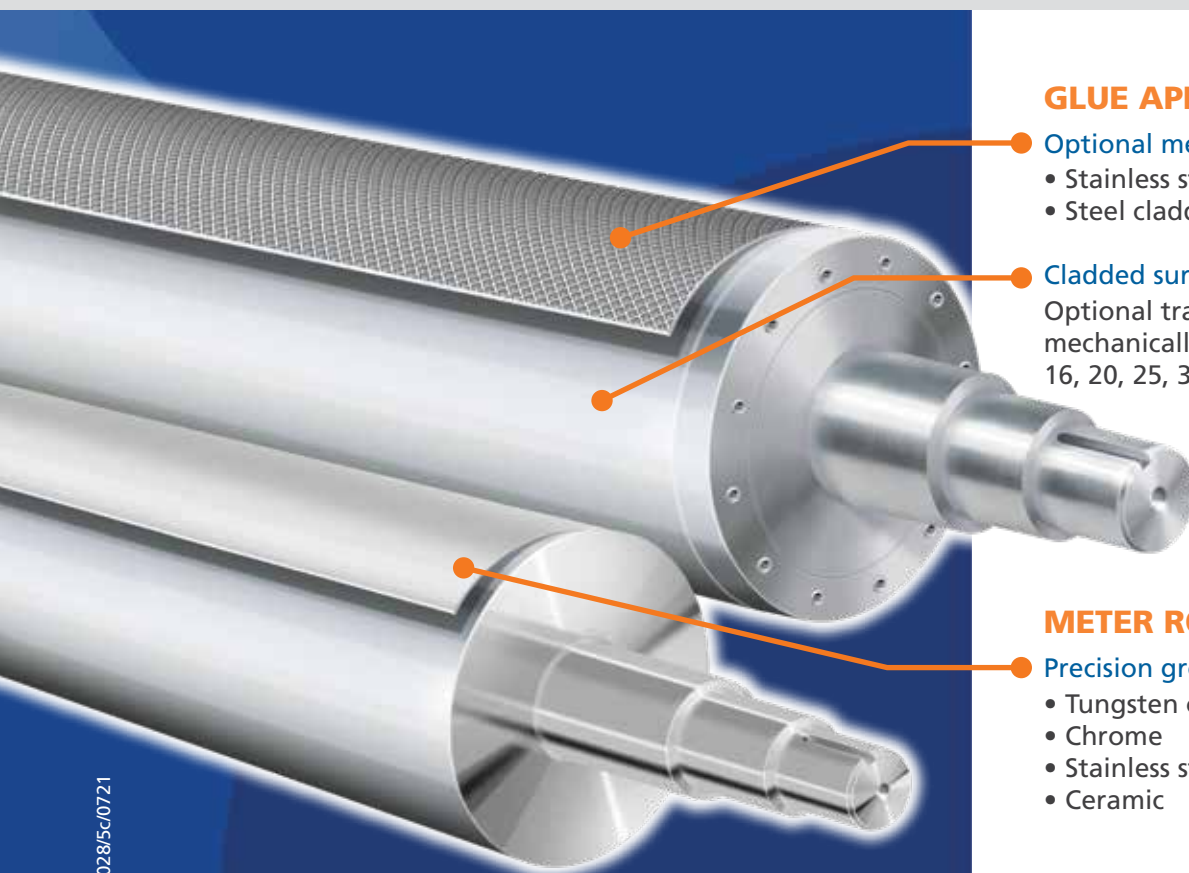
Cladded Stainless Steel Surface
